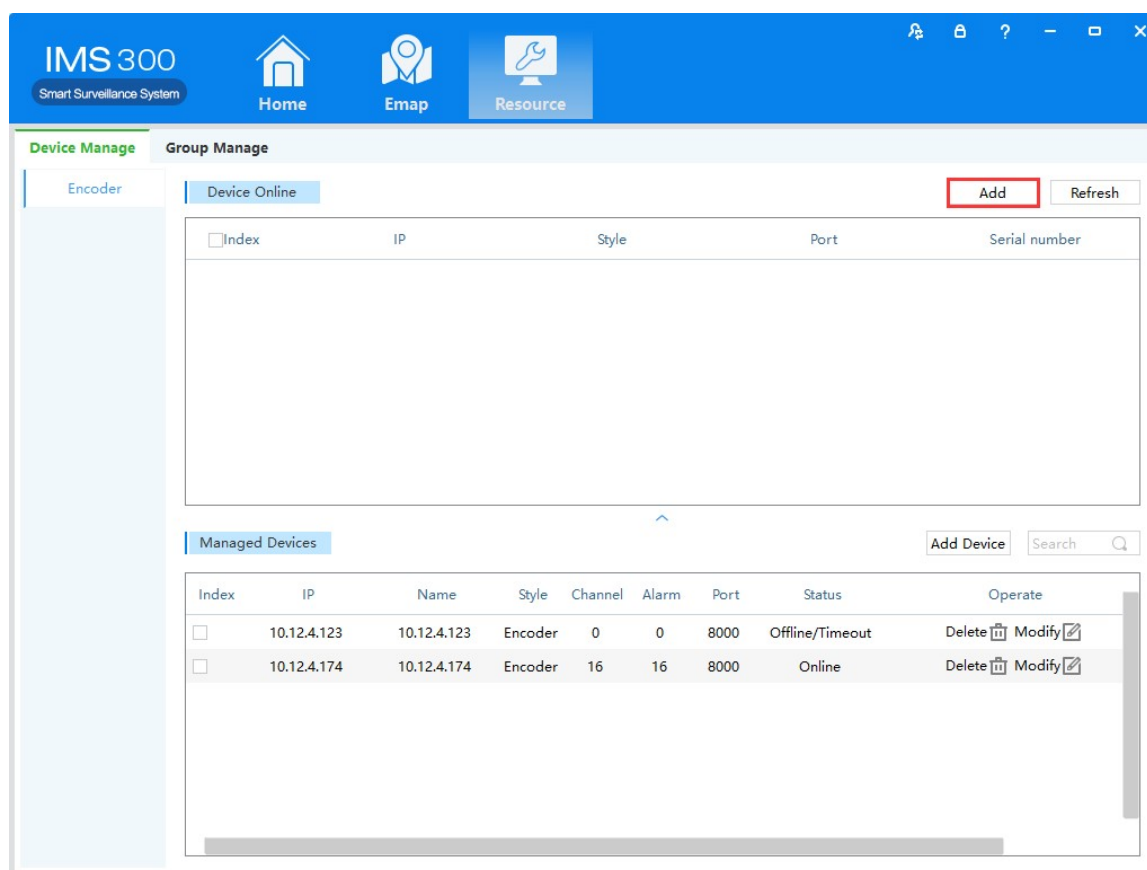
Figure 3-6 Managed Devices
