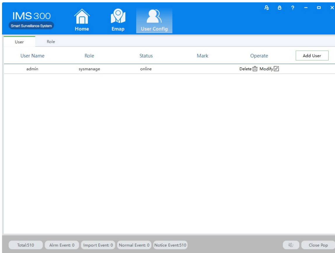
Figure 9-1 User Management
